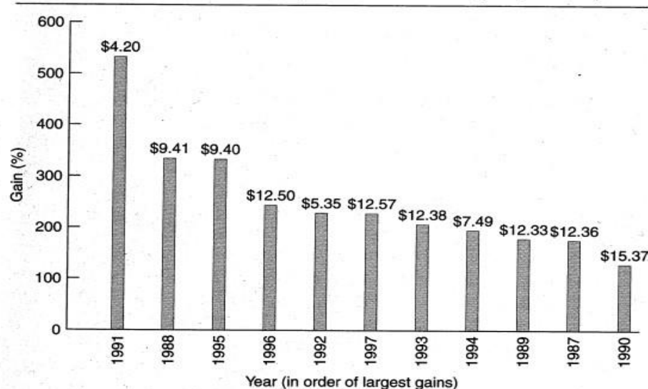
Figure 1.1 Performance of NYSE Top 10 Gains 1987-97 (price per share)
